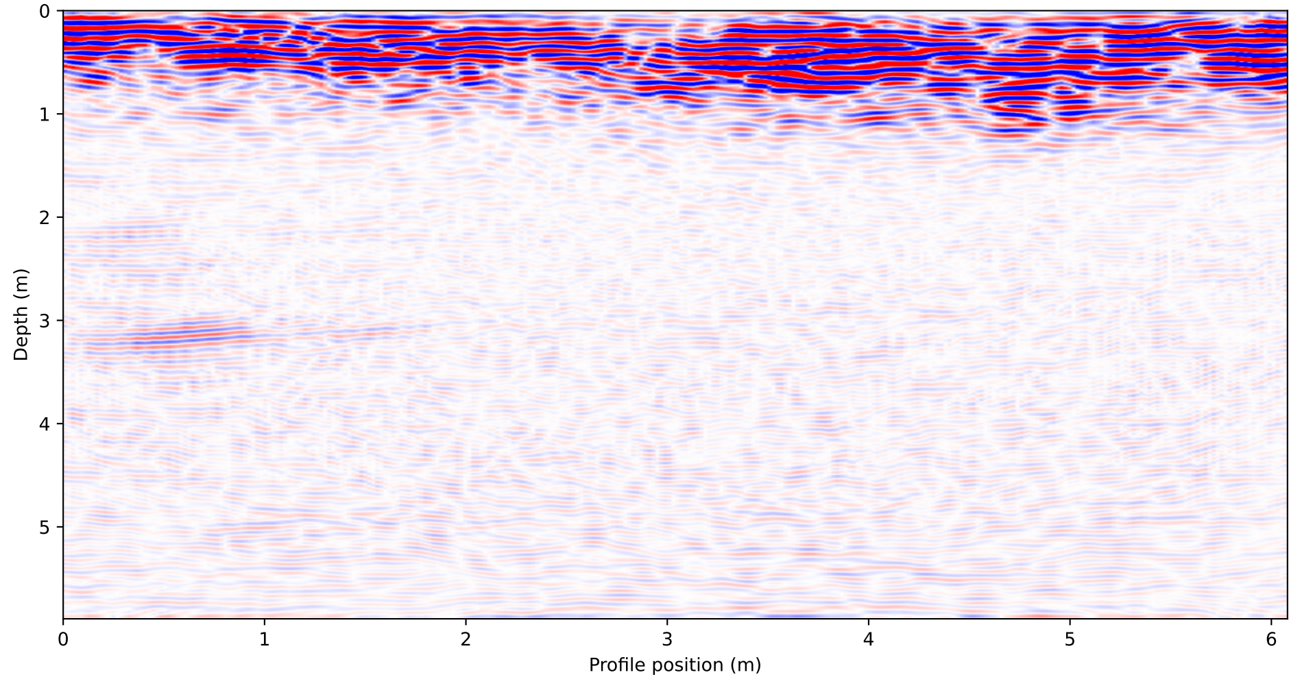
GPR Profile: line6.dt1
